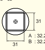
A1265B QFP 32 × 32
