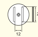
A1261B QFP 20 × 20
